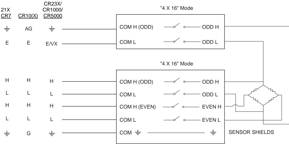
FIGURE 16. Full Bridge Measurement with Excitation Compensation
