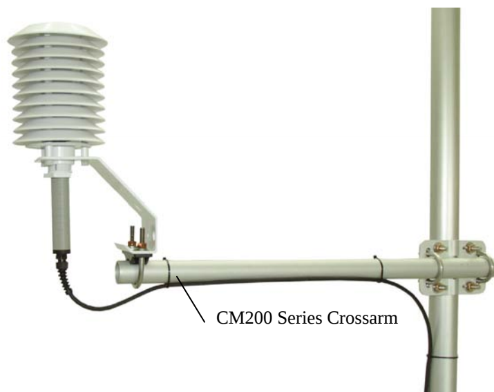
FIGURE 3-2. HMP45C and 41003-5 Radiation Shield on a CM200 Series Crossarm
