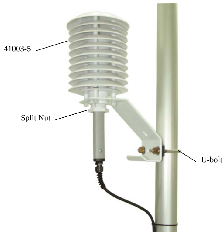
FIGURE 3-1. HMP45C and 41003-5 Radiation Shield on a Tripod Mast
