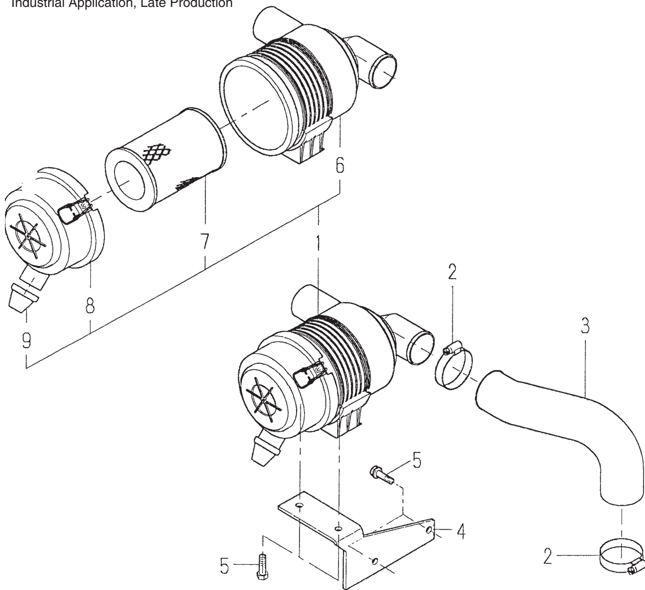
673 AIR CLEANER
